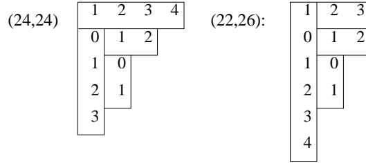
FIGURE 4. Examples: \mathcal{J}_1(024, 24) = (12234) , \mathcal{J}_1(022, 26) = (112233)
